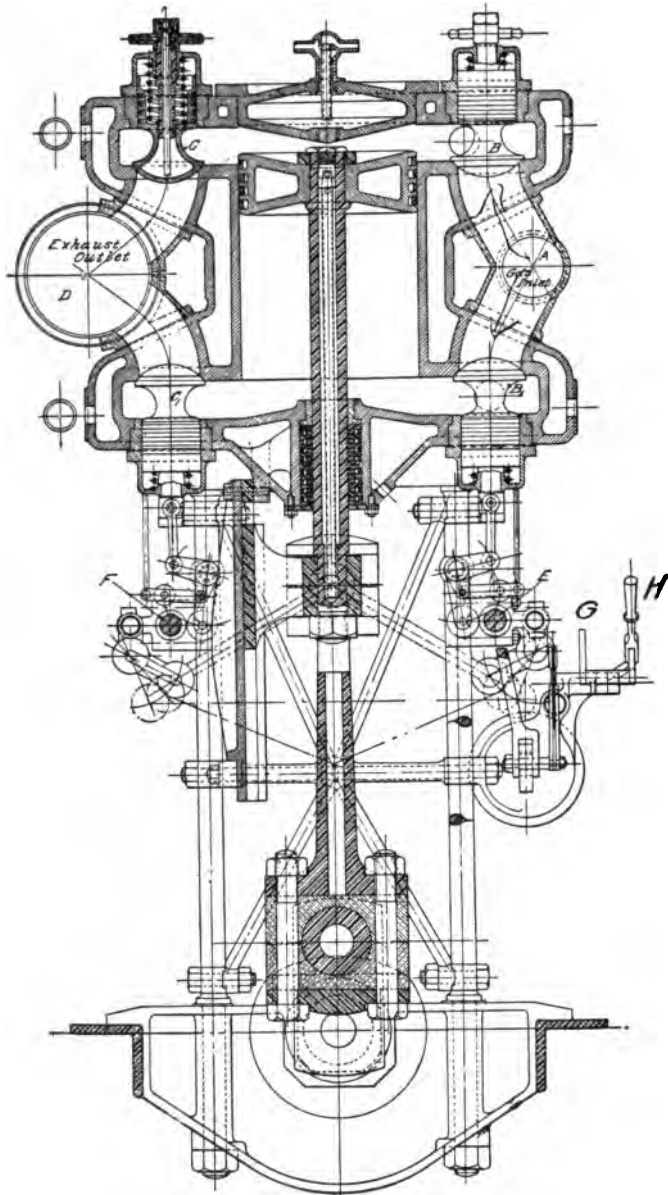
FIG. 69.—Standard Engine.
